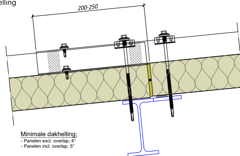
Dakhelling
